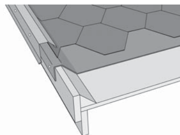
Kerabit Verge flashing for triangular batten strip
